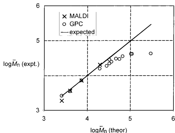
Figure 10. Points: comparison of values of \bar{M}_n predicted from the RAFT relation, eq 1, with those obtained experimentally from MALDI and from GPC using the values of K and a deduced from Figure 9. Line: values expected if all three methods gave same result.
