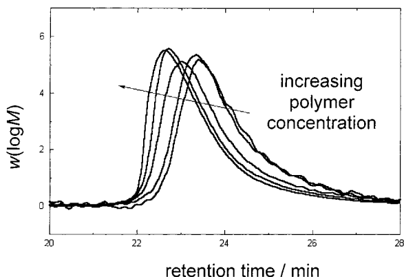
Figure 4. Influence of the polymer concentration of the control sample on the GPC chromatogram (based on polystyrene standards) of the “control” sample (no DTE). The w(\log M) are normalized by dividing the signal by the concentration. The concentration (g of polyNIPAM per \text{dm}^3 ) of each sample are the following (from top to bottom): 4.81, 2.40, 0.928, 0.96, and 0.204.
